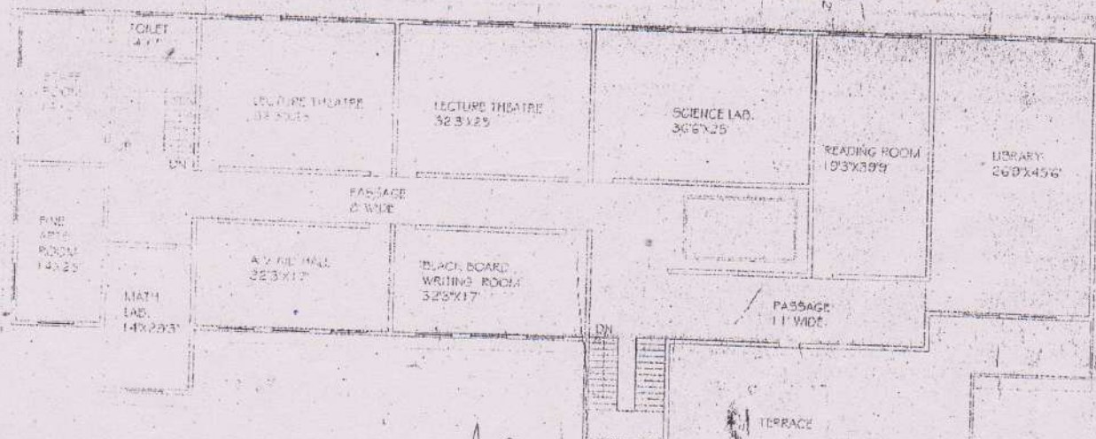
FIRST FLOOR PLAN COVERED AREA FLOOR - 9800 SQFT
